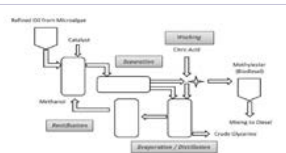
Figure 3: Schematic of esterification process of microalgal oil to biodiesel.
