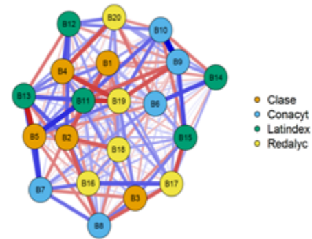
Figure 1: Network.
