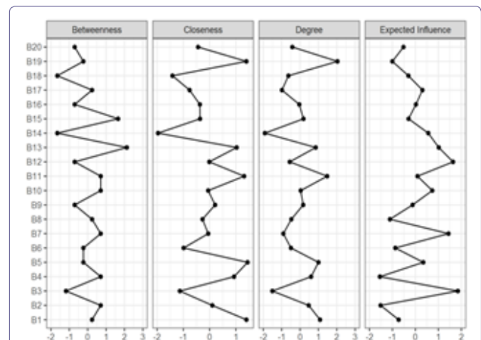
Figure 2: Centrality.
